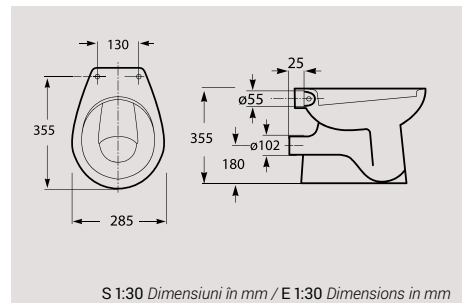
S 1:30 Dimensiuni in mm / E 1:30 Dimensions in mm
